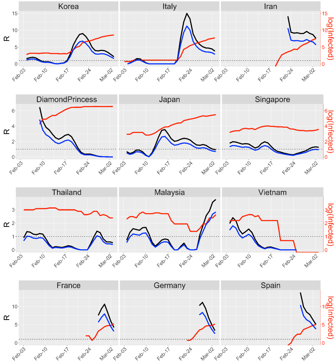
Figure 1. Time series plots of estimated effective reproduction numbers R and the logarithm of infected cases (red) up to March 2, 2020. Two R s are given based on 10.5-day infectious duration (blue) and 14-day duration (black). The critical threshold level R=1 is the horizontal dashed line.
